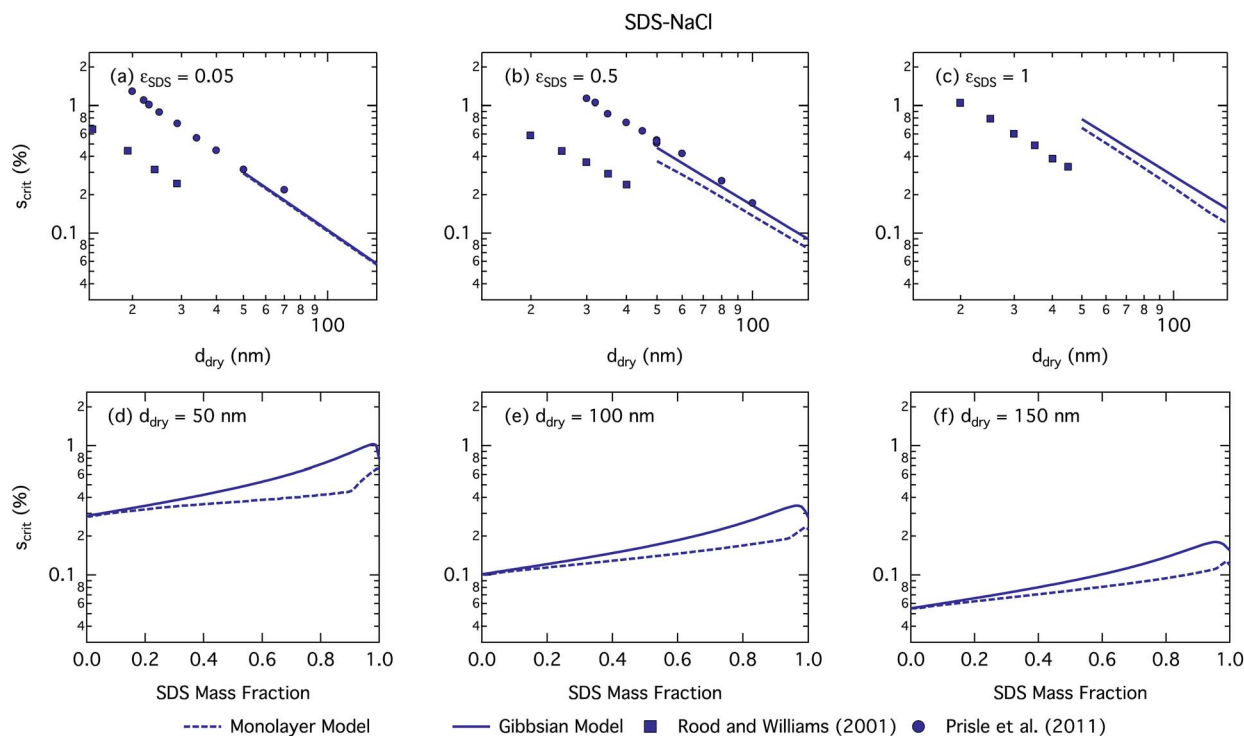
Fig. 5 Critical supersaturations calculated with the monolayer and Gibbs models as a function of dry particle size for SDS mass fractions (a) 0.05; (b) 0.5; (c) 1 and as a function of SDS mass fraction for dry particle sizes (d) 50 nm; (e) 100 nm; and (f) 150 nm. Measured critical supersaturations as a function of dry particle size from Rood and Williams 19 and Prisle et al. 6 are also shown in panels (a)–(c). The measurements in panel (a) are for pure NaCl and are shown for comparison.
