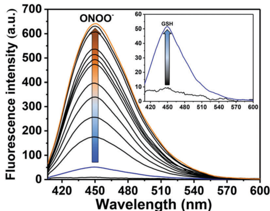
Fig. 3 Fluorescence spectra of GSH-ABAH ( 2 \mu\text{M} ) with addition of GSH ( 5 \mu\text{M} ), 1 min wait (inset), then addition of \text{ONOO}^- ( 0\text{--}14 \mu\text{M} ) in buffer solution [8% DMSO, 1 mM CTAB] ( \text{pH} = 8.20 at 25^\circ\text{C} ) fluorescence intensities were measured with \lambda_{\text{ex}} = 390 \text{ nm}/\lambda_{\text{em}} = 451 \text{ nm} with slit widths ex slit: 4 nm and em slit: 4 nm.
