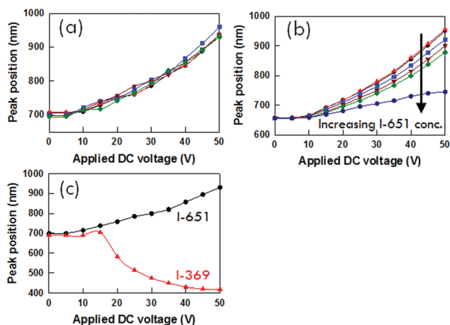
Fig. 6 (a) The position of the minimum in the selective reflection as a function of applied DC voltage of PSCLCs prepared with 250 \text{ mW cm}^{-2} of 365 nm irradiation exposure of 5 min, 10 min, 15 min, 30 min, and 60 min. (b) The position of the minimum in the selective reflection as a function of applied DC voltage of PSCLCs prepared with 250 \text{ mW cm}^{-2} of 365 nm irradiation over 30 min. PSCLCs samples were formulated with 0.1 wt%, 0.25 wt%, 0.5 wt%, 1 wt%, 2.5 wt%, and 5 wt% of I-651. (c) The position of the minimum in the selective reflection of two PSCLCs prepared from either 1 wt% I-369 or I-651 under identical exposure conditions are compared.
