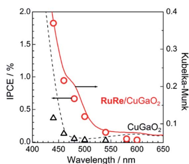
Fig. 2 Dependence on wavelength of the incident-photon-to-current efficiencies of the RuRe / CuGaO 2 (red circles) and bare CuGaO 2 (black triangles) electrodes at -0.3 V vs. \text{Ag/AgCl} . An aqueous solution containing 50 mM \text{NaHCO}_3 saturated with \text{CO}_2 was used as the electrolyte (pH 6.6). The diffuse reflectance spectra of these electrodes are also shown: RuRe / CuGaO 2 (red solid line) and CuGaO 2 (black broken line).
