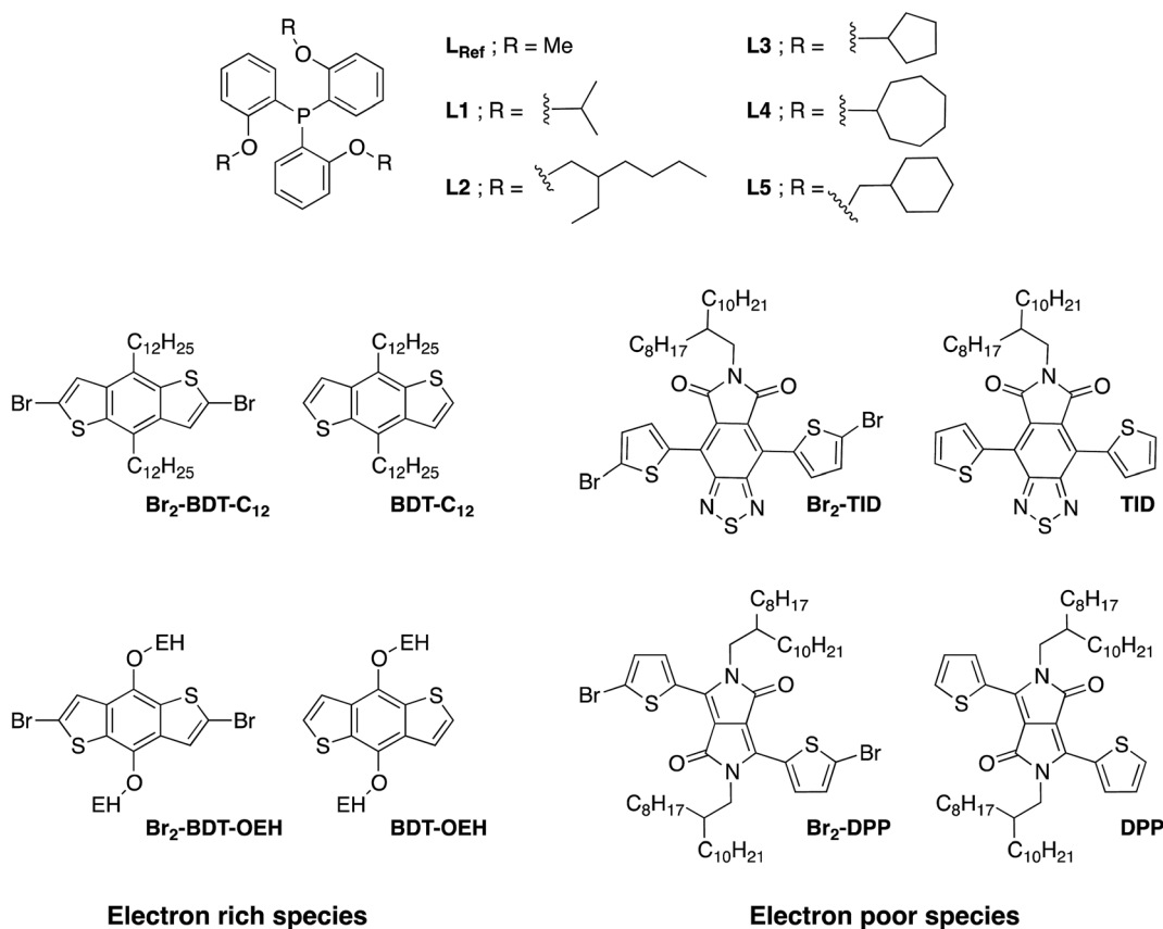
Fig. 2 The chemical structures of the phosphines and comonomers studied in this work.
