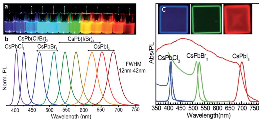
Fig. 9 (a) Colloidal perovskite CsPbX 3 NCs (X = Cl, Br, I) solutions in toluene under an UV lamp ( \lambda = 365 nm); (b) representative PL spectra ( \lambda_{\text{exc}} = 400 nm for all but 350 nm for CsPbCl 3 nanocrystals). (c) Optical absorption and PL spectra of CsPbCl 3 , CsPbBr 3 , and CsPbl 3 nanoplatelets. Inset: PL image of CsPbCl 3 , CsPbBr 3 , and CsPbl 3 nanoplatelets. Reprinted with permission from ref. 40 and 49, copyright 2015, American Chemical Society and 2016, Advanced Material.
