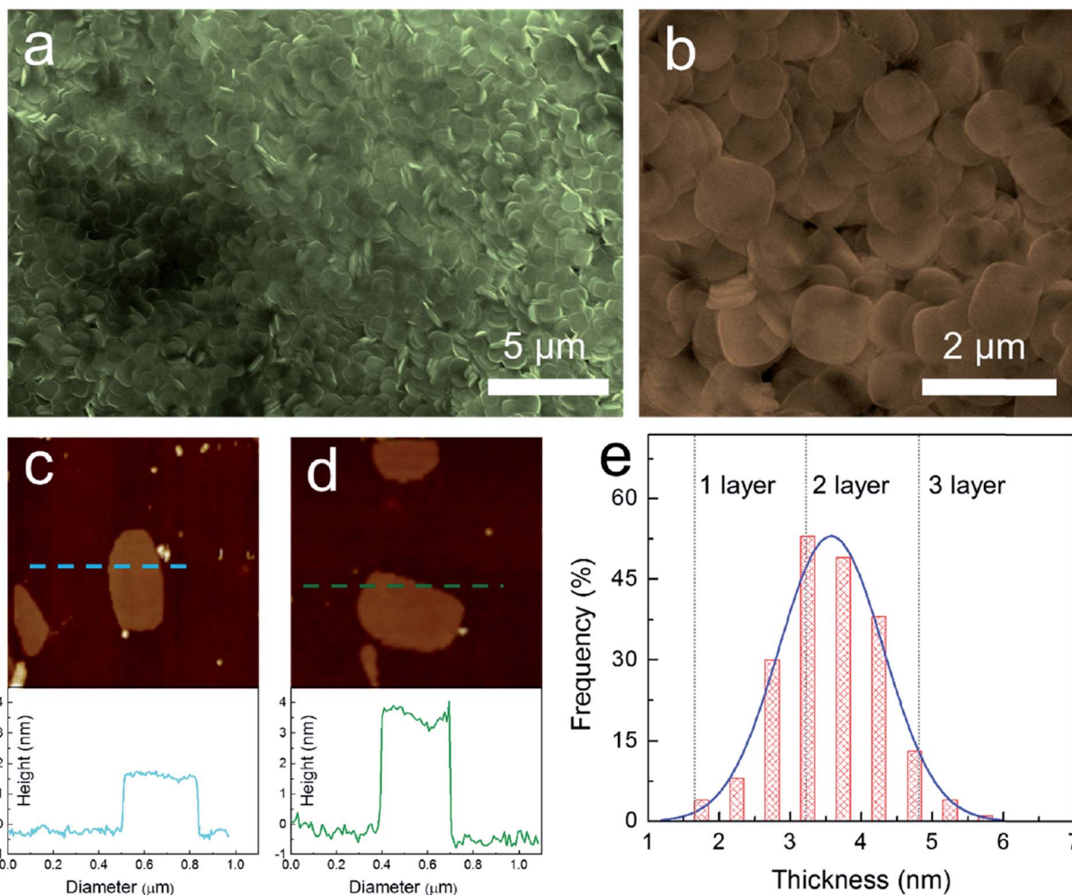
Fig. 8 Synthesis of 2D ultrathin CsPbBr 3 nanosheets: (a) low-magnification and (b) high-magnification SEM images. AFM image and height profile of (c) monolayer and (d) bilayer CsPbBr 3 nanosheets with a thickness of 1.6 and 3.3 ± 0.2 nm, respectively. (e) Thickness distribution histograms for CsPbBr 3 nanosheets prepared through solution-phase synthesis. Reprinted from ref. 79, copyright 2016, Advanced Materials.
