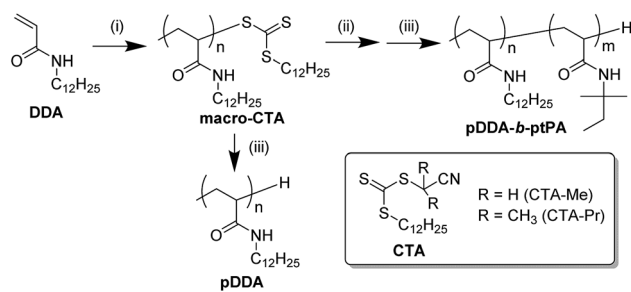
Scheme 1 Synthesis route of macro-CTA and block copolymers pDDA- b -ptPA: (i) AIBN, CTA, toluene or DMF, 60 °C, 24–48 h; (ii) tPA, AIBN, toluene, 60 °C, 20 h; (iii) tris(trimethylsilyl)silane, AIBN, toluene, 60 °C, 4 h.
