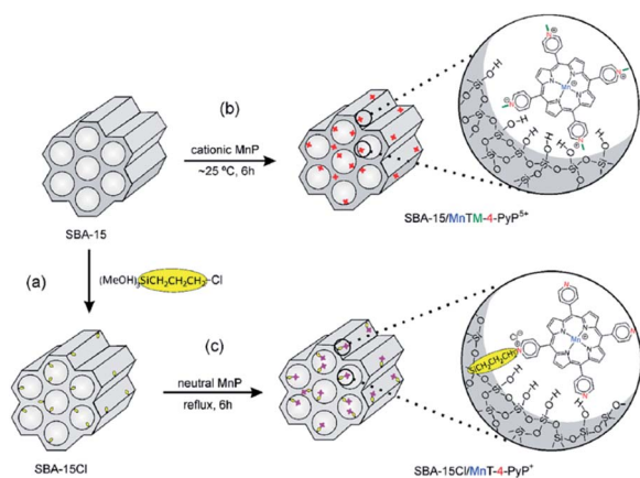
Fig. 20 Schematic representation of the synthetic routes for (a) preparation of support SBA-15Cl by the silanization of SBA-15 with (3-chloropropyl)trimethoxysilane, (b) immobilization of Mn III -TM-X-PyP + on SBA-15 by electrostatic interaction, and (c) anchorage of Mn III -T-X-PyP on SBA-15Cl by covalent bonding. The two classes of heterogenized catalysts are illustrated with the para MnP isomers. Reprinted from ref. 118 with permission of Elsevier.
