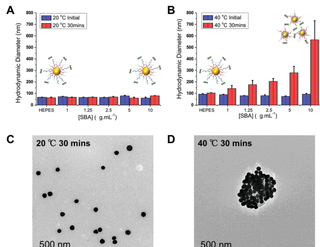
Fig. 3 Dynamic light scattering (DLS) analysis of thermally gated lectin binding. pHEA 15 -Gal : pNIPAM 50 ratio 9 : 1 @ AuNP 60 . (A) Hydrodynamic diameter at 20 °C initially, and after 30 minutes incubation with SBA; (B) hydrodynamic diameter at 40 °C, initially and after 30 minutes incubation with SBA. All results are mean from a minimum of 3 independent repeats. TEM images of these particles after addition of SBA ( 10\ \mu\text{g mL}^{-1} ): (C) at 20 °C for 30 min; (D) at 40 °C following 30 minutes incubation.
