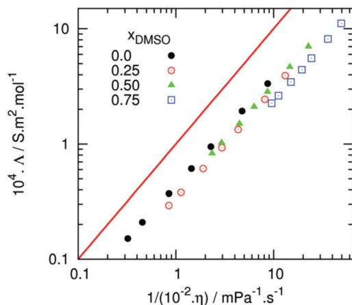
Fig. 8 Walden plot comparing the viscosity and conductivity values for binary [\text{C}_4\text{C}_1\text{im}][\text{OAc}] -DMSO mixtures ( \chi_{\text{DMSO}} = 0, 0.25, 0.5, 0.75 ), reproduced from ref. 107 with permission from the Royal Society of Chemistry. The red line denotes the reference ionicity of 0.01 M aqueous KCl, at 25 °C.
