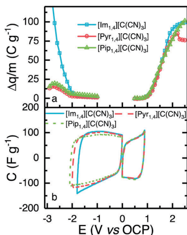
Fig. 4 Electrochemical stability window determination. (a) difference between q_{\text{charge}} and q_{\text{discharge}} . (b) CV at determined limit voltage for positive and negative sweep for the ILs [Im 1,4 ][C(CN) 3 ] (blue), [Pyr 1,4 ][C(CN) 3 ] (red) and [Pip 1,4 ][C(CN) 3 ] (green).
