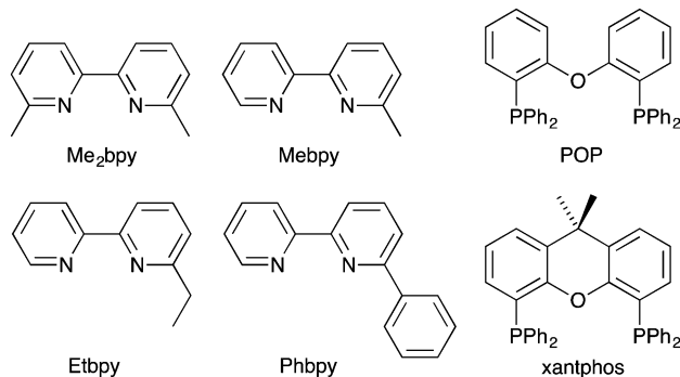
Scheme 1 Structures of \text{N}^{\wedge}\text{N} ligands 6,6'-dimethyl-2,2'-bipyridine ( Me 2 bpy ), 6-methyl-2,2'-bipyridine ( Mebpy ), 6-ethyl-2,2'-bipyridine ( Etbpy ) and 6-phenyl-2,2'-bipyridine ( Phbpy ), and the \text{P}^{\wedge}\text{P} ligands POP and xantphos .
