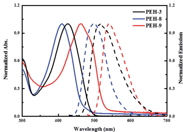
Fig. 2 UV-vis absorption (solid line) and emission (dashed line) spectra of PEH-3 (black), PEH-8 (blue) and PEH-9 (red) in dichloromethane.
