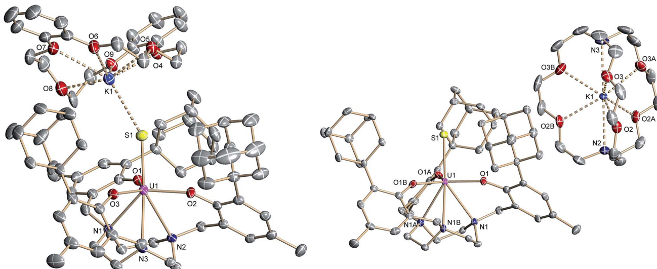
Fig. 2 Molecular structure of the uranium(IV) sulfido complex [(^{Ad,Me}ArO)_3tacn)U\equiv S \cdots K(db-18-c-6)] ( 3 ) (left), and [K(2.2.2-crypt)][(^{Ad,Me}ArO)_3tacn)U\equiv S] ( 4 ) (right). All hydrogen atoms and the solvent molecules are omitted for clarity (50% probability ellipsoids).
