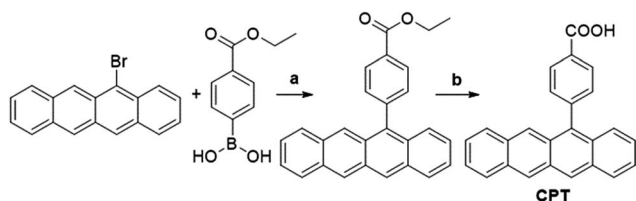
Scheme 1 Synthesis of transmitter tetracene derivative 4-(tetracene-5-yl)benzoic acid (CPT). Reagents and conditions: (a) \text{Cs}_2\text{CO}_3 , \text{Pd}(\text{dppf})\text{Cl}_2 \cdot \text{CH}_2\text{Cl}_2 , toluene : \text{H}_2\text{O} = 3 : 1 , 60^\circ\text{C} , overnight. (b) 2 M KOH aqueous solution, THF : MeOH = 1 : 1, reflux, 3 h.
