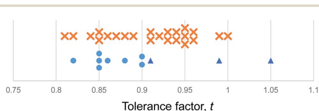
Fig. 1 The tolerance factors of ABI_3 compounds. Blue dots represent inorganic ABI_3 compounds that form perovskites at room temperature and pressure. Red crosses represent inorganic ABI_3 compounds that do not form perovskites. Blue triangles show hybrid APbI_3 and ASnI_3 compounds that form in the perovskite structure, using the methodology of Cheetham et al. to estimate molecular ion radii. 26,27 There is no boundary on the tolerance factor scale that separates perovskites from non-perovskites.
