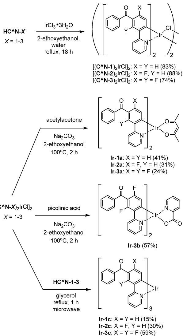
Scheme 2 Syntheses of iridium(III) complexes.
