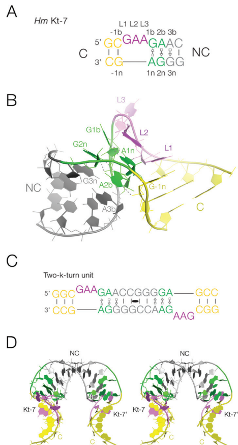
Fig. 1 The k-turn, and the two-k-turn unit. A , The sequence of Kt-7, a standard simple k-turn. The standard nomenclature of the nucleotide positions is shown. The color scheme for the nucleotides is followed in all the structures shown subsequently. B , The structure of a single Kt-7 k-turn, taken from structure PDB 4CS1. In the view shown the loop of the k-turn (colored purple) is at the back, and the NC helix with the G-A pairs is on the left. C , The sequence of the two-k-turn unit. A self-complementary RNA forms a duplex structure with two Kt-7 k-turns related by a central two-fold axis of rotational symmetry. The two k-turns are connected through their common NC helix (grey), and the two C helices (yellow) form the termini. D , A parallel-eye stereoscopic view of the structure of the two-k-turn unit taken from structure PDB 4CS1.
