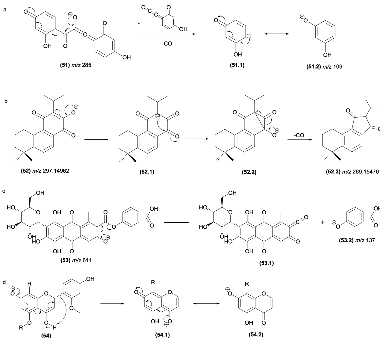
Fig. 27 \alpha -Eliminations resulting in the loss of \text{CO} in flavonoids (a) and abietane-type diterpenes. \gamma -Elimination in anthraquinones (c) and \zeta -elimination in flavonoids (d).
