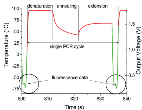
Fig. 3 PCR thermal profile of a single amplification step. The heater temperature (red part) is linearly proportional to the built-in lock-in amplifier output, which was captured with an oscilloscope. While performing denaturation at \approx 93 °C, annealing at \approx 56 °C and most of the extension step at \approx 72 °C, the built-in lock-in amplifier is utilized to measure the average temperature of all four heaters. In the last two seconds of the extension step, the lock-in amplifier is used to sequentially process the fluorescence signal (green part) from the 4 measurement spots (circled area). These data are stored in their original format in analog-to-digital converter units (ADC units) within the memory of a microcontroller. Once fluorescence is measured, the heater is powered by the average value of pulse width modulation obtained during the extension phase.
