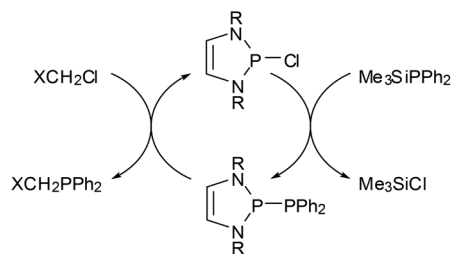
Scheme 7 DAP-catalyzed phosphorus carbon cross coupling reaction (according to ref. 45; X = Cl, CN, Ph, C 3 H 7 , yields 80–99%).
