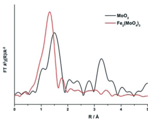
Fig. 11 Magnitude component of the k^2 weighted Fourier Transform data for MoO 2 and Fe 2 (MoO 4 ) 3 (Sigma Aldrich).
