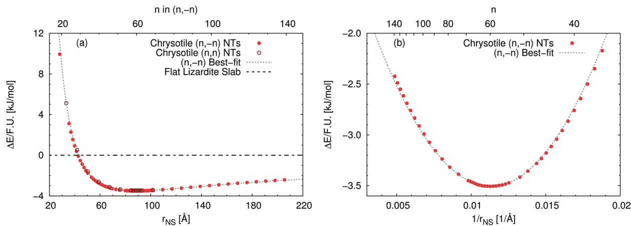
Fig. 3 Energy difference per formula unit of (n, -n) single-walled chrysotile nanotubes with respect to the flat lizardite slab [ \text{kJ mol}^{-1} ], as a function of (a) NS radius [Å] and index n , and (b) inverse NS radius [ \text{Å}^{-1} ] and index n . The superimposed curve has been obtained through quadratic best-fit over a set of 16 points around the energy minimum. In (a), data for the (n, n) series are also shown. In (b), only the subset of (n, -n) data in the energy range of -3.6 – -2 \text{kJ mol}^{-1} is shown. All the corresponding (n, -n) data are reported in Table S1 in the ESI.†
