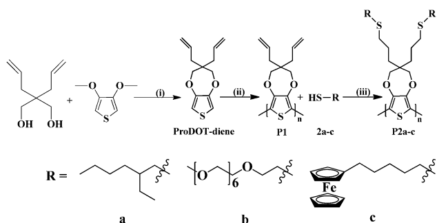
Scheme 1 Synthesis of ProDOT-diene ( 1 ), electrochemical polymerization of ( 1 ) to form poly(ProDOT-diene) ( P1 ) and “click” reaction of P1 with various thiols 2a-c to form P2a-c . (i) p -TSA in toluene at 100 ^\circ\text{C} for 2 days (ii) ACN-TBAP; (iii) 0.1% DMAP, UV 365 nm, room temperature.
