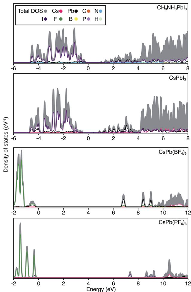
Fig. 3 Electronic density of states are shown for CH 3 NH 3 PbI 3 , CsPbI 3 , CsPb(BF 4 ) 3 and CsPb(PF 6 ) 3 . The top of the valence band is set to 0 eV in each case, and the partial ion contributions are determined from a spherical integration around each lattice site. The similarity between the electronic structure for Cs and CH 3 NH 3 compounds has previously been noted. 30 For the polyanion compounds, the band gaps are widened and the band edges become more localized, in accordance with the band structures shown in Fig. 2.
