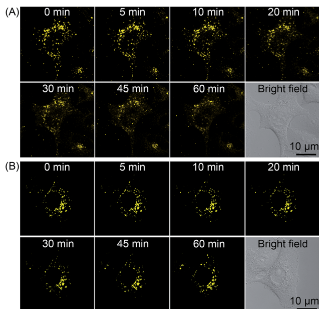
Fig. 10 Real-time monitoring of lysosomal integrity in A549 cells loaded with 2 (10 \mu\text{M} , 12 h) (A) with or (B) without PDT treatment (120 s, 4.8 J cm -2 ).
