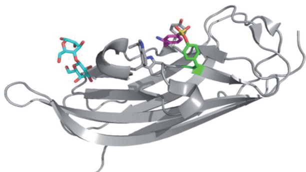
Fig. 5 AEBSF (magenta) adduct of dscPsaA in complex with galactose (cyan) (PDB 4F8O).
