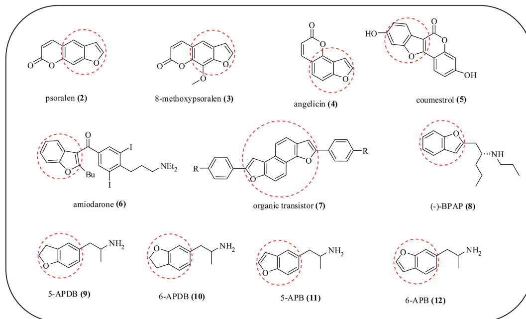
Fig. 2 Benzofuran core, a multifunctional nucleus.
