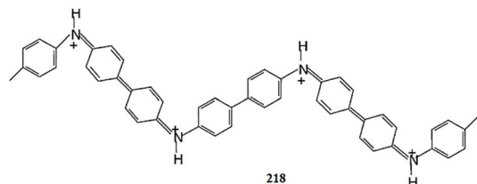
Fig. 182 Bipolaronic form of PDPA 218.
