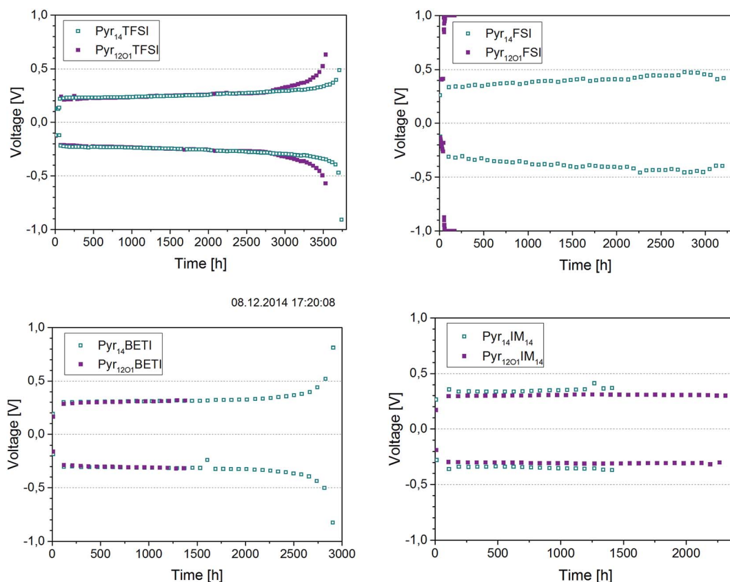
Fig. 9 Stripping–plating in symmetrical lithium cells at 0.1\text{ mA cm}^{-2} and 40^\circ\text{C} . The ionic liquid present in the electrolytes is indicated in the legends.
