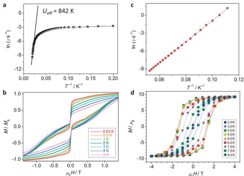
Fig. 14 Experimental data for polynuclear dysprosium(III)-based single molecule magnets. (a) Arrhenius plot and (b) hysteresis plot for [(\text{Dy}_3\text{Y})_4\text{K}_2\text{O}(\text{OtBu})_{12}] recorded at a sweep rate of 0.14 \text{ T s}^{-1} , adapted by permission from Macmillan Publishers Ltd, ref. 8, copyright 2013; (c) Arrhenius plot and (d) hysteresis plot for [\text{K}(18\text{-crown-6})]\{[(\text{Me}_3\text{Si})_2\text{N}]_2(\text{THF})\text{Dy}\}_2(\mu\text{-}\eta^2:\eta^2\text{-N}_2) , recorded at a sweep rate of 0.08 \text{ T s}^{-1} , adapted by permission from Macmillan Publishers Ltd, ref. 42, copyright 2011.
