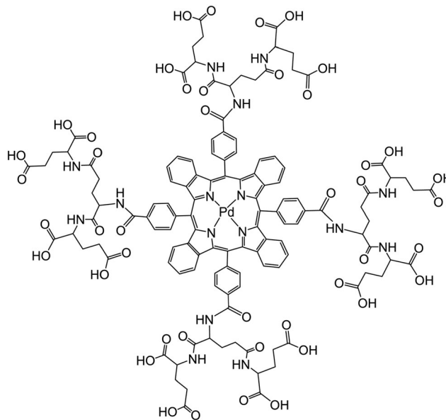
Fig. 7 Chemical structure of the dendrimeric nanoparticles used (under the tradename Oxyphore G ) for imaging of oxygen. It consists of a Pd(II)benzoporphyrin core and a glutamate-based periphery whose carboxy groups are dissociated which imparts water solubility. From ref. 174 with permission (2014) by Springer Verlag (Berlin).
