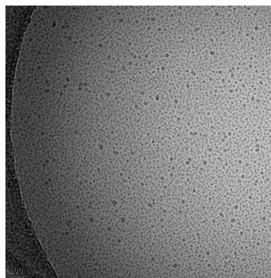
Fig. 2 Cryo-TEM image of micelles formed by daptomycin (2.5 mM in 0.625 mM CaCl 2 ). 18
