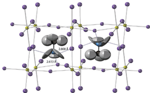
Fig. 1 The unit cell of MAPbI 3 at 100 K viewed close to a -axis showing ADPs as 90% probability ellipsoids; lead yellow, iodine purple, carbon black, nitrogen blue and hydrogen grey.
