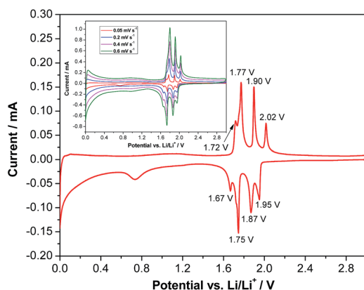
Fig. 2 Cyclic voltammogram of LVP anodes recorded at a scan rate of 0.05 \text{ mV s}^{-1} in the potential range of 3.0–0.0 V vs. \text{Li}/\text{Li}^+ . Inset: CV at different scan rates.
