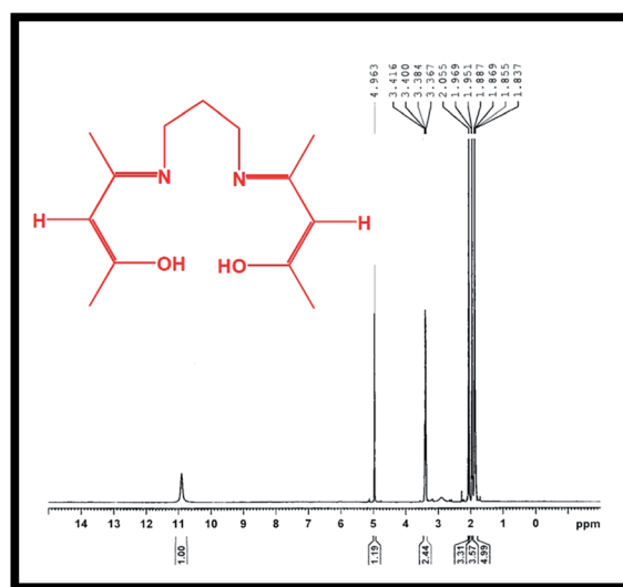
Fig. 2 1 H-NMR of the H 2 (pnAA 2 ) Schiff-base.
