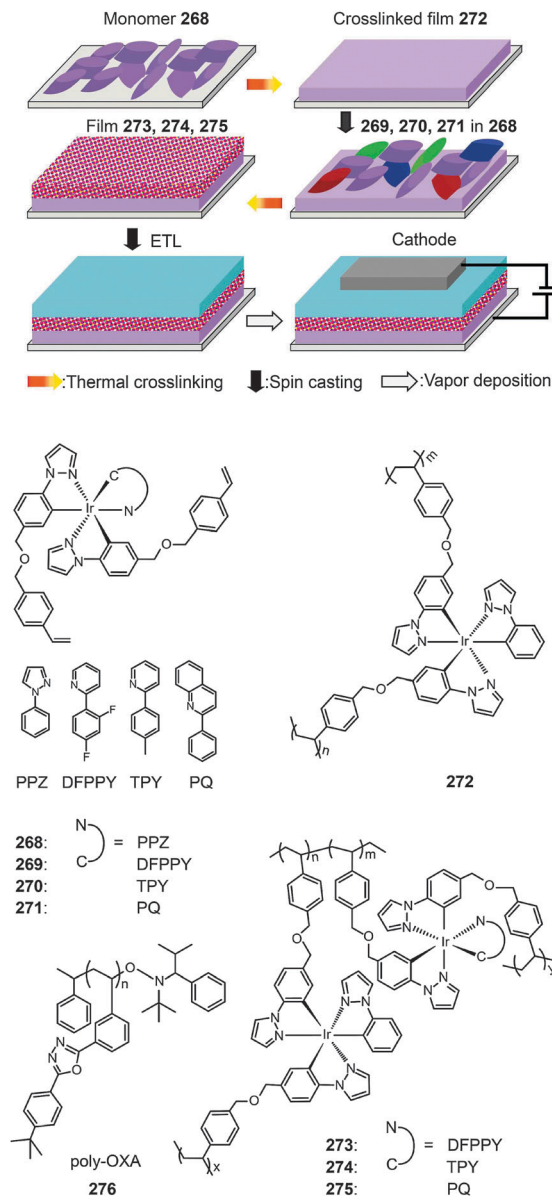
Fig. 18 procedure of solution-processed multi-layer devices on the basis of crosslinkable monomers 268–271 and the corresponding crosslinked polymeric polymers 272–275. (Reproduced with permission from ref. 116. Copyright 2009, Wiley-VCH Verlag GmbH & Co. KGaA.)
