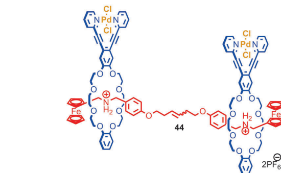
Fig. 23 Osakada's [3]rotaxane Pd catalyst for the Mizoroki–Heck reaction.
