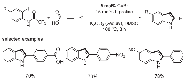
Scheme 41 Synthesis of 2-arylidoles.
