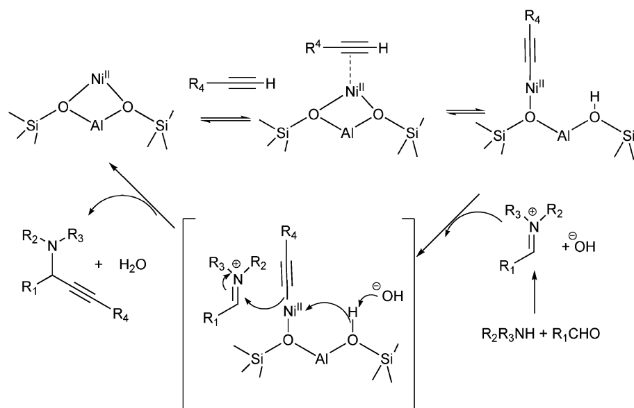
Scheme 4 Possible mechanism of \text{Ni}^{\text{II}}\text{-Y} -catalyzed three component coupling.
