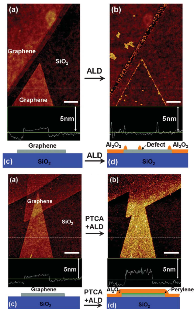
Fig. 7 ALD of Al 2 O 3 on (Top) pristine GN and (Bottom) PCTA-coated GN. (a) Atomic force microscopy (AFM) image of GN on SiO 2 before ALD. (b) AFM image of the same area as (a) after Al 2 O 3 ALD deposition. (c) and (d) Schematics of GN on SiO 2 before and after ALD. Reprinted with permission from ref. 330. Copyright 2008, American Chemical Society.
