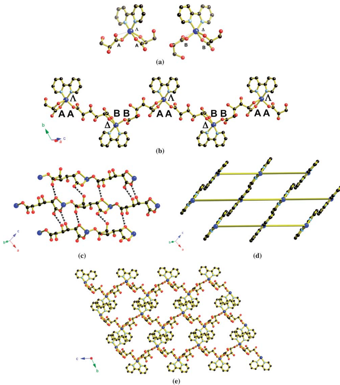
Fig. 4 The structure of Cu(sac)(bipy). (a) The coordination environments of the two types of Cu(II) centre in the structure. (b) A section of the 1D zig-zag coordination polymer. (c) Part of the hydrogen bonded sheet formed from chains linked from hydrogen bonding (indicated by striped connections). The sheet is parallel to the a - c plane. Bipy ligands are not shown. (d) Part of the 2D sheet indicating the orientations of the bipy ligands. Bridging saccharate ligands are indicated by long connections. (e) The 3D structure viewed edge-on to the 2D sheets. Channels running parallel to the b direction lie between the interdigitating bipy ligands. Colour code: see Fig. 1 caption; Cu blue. Hydrogen atoms have been omitted for clarity.
