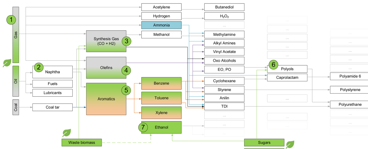
Fig. 12 Selected examples of value chain entry points for biomass at the stage of basic raw material (biomethane, 1, or bionaphtha, 2), primary building block (syngas, 3) or directly as functional building blocks, e.g. sugars or plant oil as multi-functional monomers (6) used in polyol production, copolymerized with ethylene oxide (EO) and propylene oxide (PO), as building block for polyurethanes. Note, that entry points can be combined: the EO and PO in this example could stem from bionaphtha (2). New transformation technologies, based on gasification of biomass and conversion to olefins (4) or aromats (5) further add possibilities to connect chemical value chains to renewable raw material sources. Bioethanol (7) can be another starting point of C2 value chains, which can be connected or independent on fossil chains.
