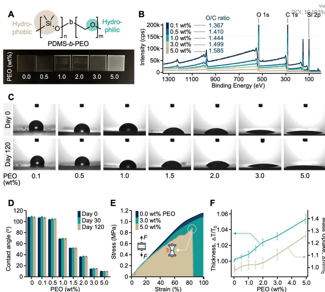
Figure 2. Amphiphilic and functional properties of PDMS-(PDMS-b-PEO) composites. (a) General molecular structure of PDMS-b-PEO copolymer, exhibiting amphiphilic characteristics with hydrophobic PDMS and hydrophilic PEO blocks (top); Optical images of PDMS-(PDMS-b-PEO) composites showing increased opacity with higher PEO content (bottom). (b) XPS spectra of composites with varying PDMS-b-PEO concentrations, confirming incorporation of PEO domains and corresponding elemental signals (O 1s, C 1s, Si 2p). (c) Representative water contact angle images at Day 0 and Day 120 across different PEO concentrations (0.1–5.0 wt%). (d) Quantified contact angle values over time (day 0, 30, and 120), measured under dry storage conditions, showing enhanced and sustained hydrophilicity with increasing PDMS-b-PEO content. (e) Stress-strain curves of composites with different PDMS-b-PEO concentrations, indicating reduced mechanical stretchability at \geq 5.0 wt% PEO (film rupture observed with notched samples). (f) Swelling behavior after 90-day immersion in artificial saliva: Normalized thickness change ( \Delta T/T_0 , left axis) and normalized mass uptake ( \Delta m/m_0 , right axis) increase with PEO concentration, confirming partial water absorption by PEO domains.
