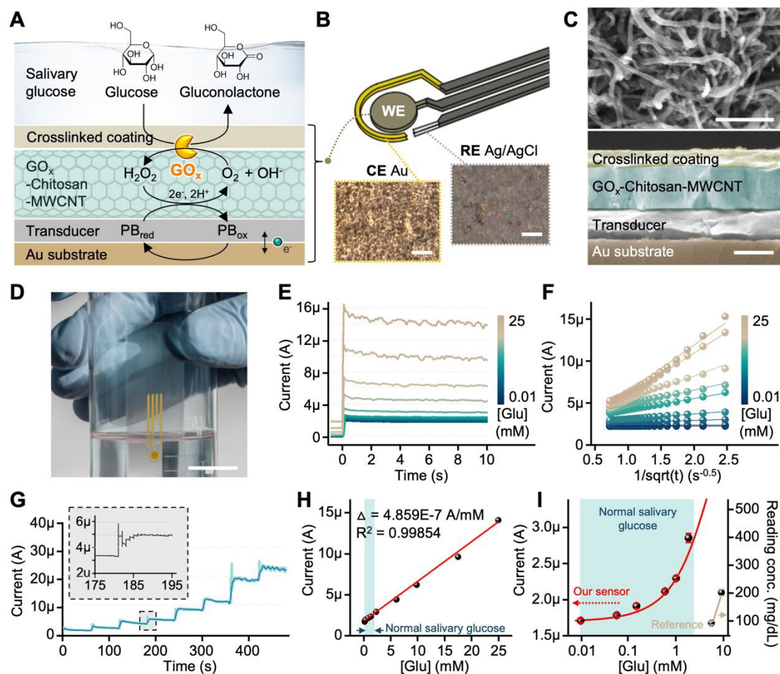
Figure 3. Structural design and electrochemical performance of the salivary glucose sensor. (a) Schematic illustration of the glucose oxidation and detection mechanism at the GOx-based working electrode. Glucose is catalytically oxidized to gluconolactone, generating \text{H}_2\text{O}_2 , which is further decomposed to release electrons for signal transduction. (b) Configuration of the three-electrode system (working (WE), reference (RE), and counter electrodes (CE)), with corresponding optical micrographs of the RE and CE. Scale bar = 50 \mu\text{m} . (c) (Top) FE-SEM image of the multi-walled carbon nanotube (MWCNT) network structure; (Bottom) Cross-sectional SEM image of the working electrode, revealing layered construction: Au substrate, transducer, GOx–Chitosan–MWCNT, and crosslinked glutaraldehyde coating. Scale bar = 500 nm. (d) Photograph of the experimental setup used for calibration, showing the electrode immersed in glucose stock solutions. Scale bar = 2 cm. (e) Chronoamperometric current responses corresponding to various glucose concentrations (0.01–25 mM), demonstrating signal magnitude increases with glucose levels. (f) Cottrell analysis of transient current profiles, used to extract diffusion coefficients from \tau values. (g) Real-time chronoamperometric trace during stepwise glucose injections, showing discrete current steps. (h) Calibration curve derived from steady-state current vs. glucose concentration. (i) Magnified view of the calibration curve, highlighting the physiological range of normal salivary glucose for comparison and sensor validation.
