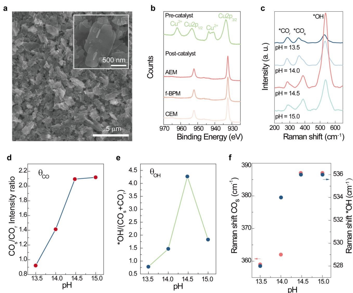
Figure 3. Cathode characterization and in situ Raman analysis. a . Scanning electron microscope image of the CuO pre-catalyst. b . High-resolution XPS spectra of the catalyst-coated gas diffusion electrode (GDE) pre- and post-electrolysis. c . Operando Raman spectra of CuNPs acquired during CORR at bulk pH 13.5-15.0 at potential
