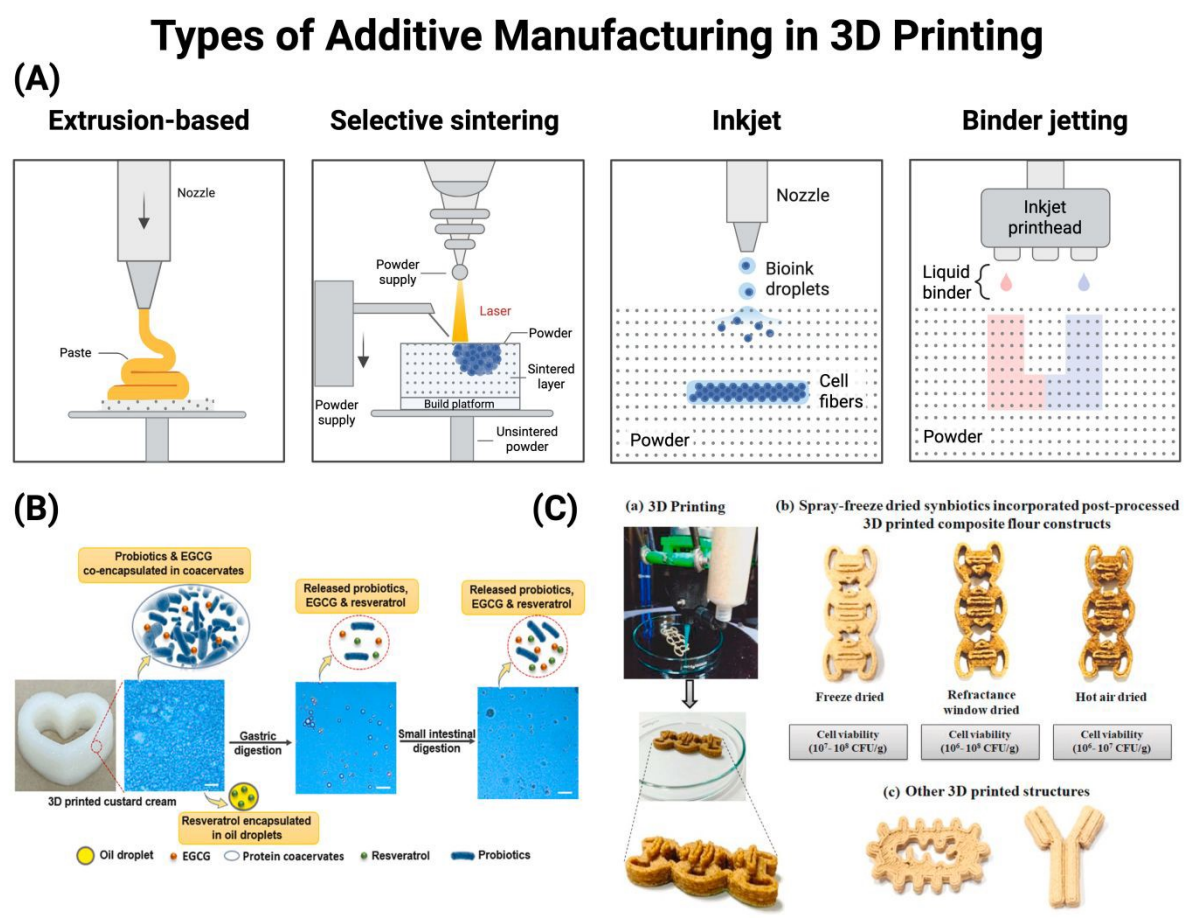
Fig. 6 (A) Schematic illustration of four main types of additive manufacturing in food 3D printing: extrusion-based printing, selective laser sintering, inkjet printing, and binder jetting (created with BioRender). (B) Custard cream prepared by extrusion-based 3D printing with co-encapsulation of probiotics, epigallocatechin gallate (EGCG), and resveratrol, reproduced from reference [79] with permission from Elsevier, copyright 2023. (C) Comparison of different drying methods applied to 3D printed Lactiplantibacillus plantarum (NCIM 2083), including freeze-drying, refractance window drying, and hot air drying, reproduced from reference [129] with permission from Elsevier, copyright 2021.
