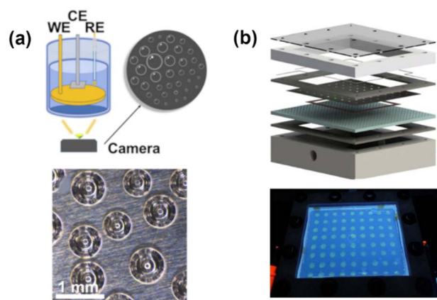
Fig. 4 (a) HT bubble screening setup for measuring HER activity with an example of the camera view below. The camera below the working electrode allows for visualization of the \text{H}_2 bubbles forming on the catalyst compositional library. WE: working electrode; CE: counter electrode; RE: reference electrode. Reproduced with permission from ref. 106. Copyright 2023 Elsevier B.V. (b) An exploded (top) and live (bottom) view of a custom, 72-sample HT cell for measuring \text{eCO}_2\text{RR} activity based on color change with a pH indicator. The authors validated the setup by depositing the same catalyst in each location and ensuring that the pH color did not vary. Reproduced with permission from ref. 101. Copyright 2021 Springer Nature Ltd.
