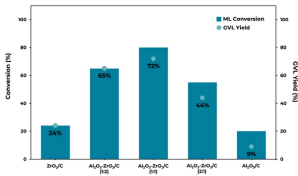
Fig. 6 Catalyst screening in the CTH of methyl levulinate into \gamma -valerolactone promoted by MOF-derived \text{Al}_2\text{O}_3 - \text{ZrO}_2 /C catalysts by using 2-propanol as an H-source (reaction conditions: 0.5 \text{ mL min}^{-1} flow rate; ML 0.2 M in 2-propanol; 0.500 g of catalyst; 30 bar pressure; time on stream: 30 min; reaction temperature: 200^\circ\text{C} ).
