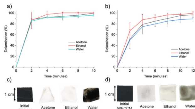
Fig. 4 Delamination percentage in water with an ultrasonic bath of (a) fuel cell CCM and (b) water electrolyser CCM after swelling in different solvents, (c) picture of fuel cell CCM and (d) water electrolyser CCM after soaking in acetone, ethanol, and water, followed by sonication in water (10 min for fuel cell CCM and 12 min for water electrolyser CCM).
