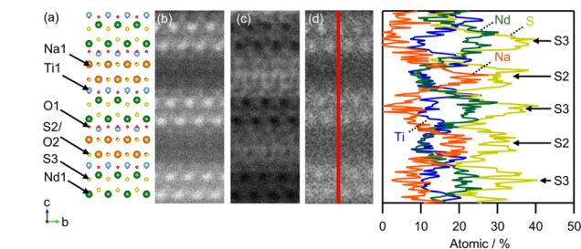
Fig. 4 STEM images of \text{NaNdTiO}_{2.2}\text{S}_{1.8} in the [100] direction. (a) The crystal structure of \text{NaNdTiO}_{2.2}\text{S}_{1.8} . Enlargements of (b) HAADF and (c) ABF. (d) STEM-EDX line analysis of \text{NaNdTiO}_{2.2}\text{S}_{1.8} .
